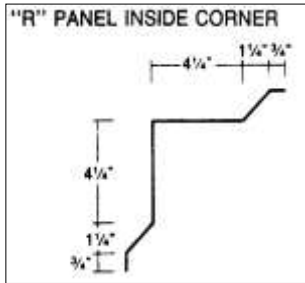
Inside Corner R-Panel
