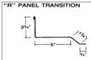
Transition Trim R-Panel
