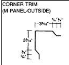
Corner trim M-Panel Outside
