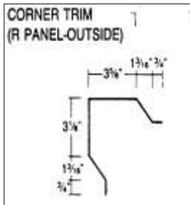
Corner trim R-Panel Outside
